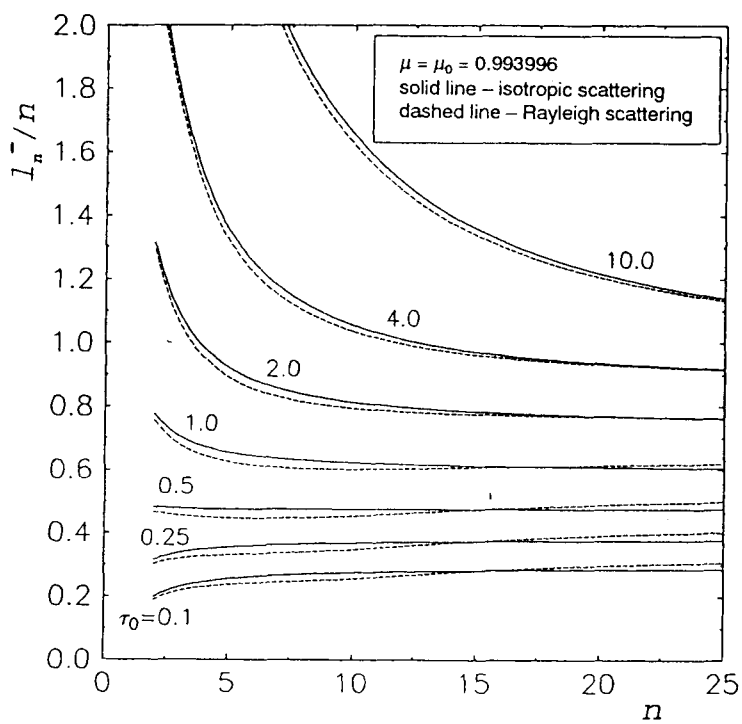
Fig. 2. Same as in Fig. 1 for transmitted radiation.
