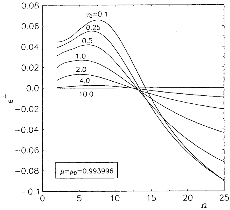
Fig. 3. Relative differences in the average path-lengths for emergent radiation at \tau = 0 for isotropically and Rayleigh scattering atmospheres as functions of the order of scattering.
