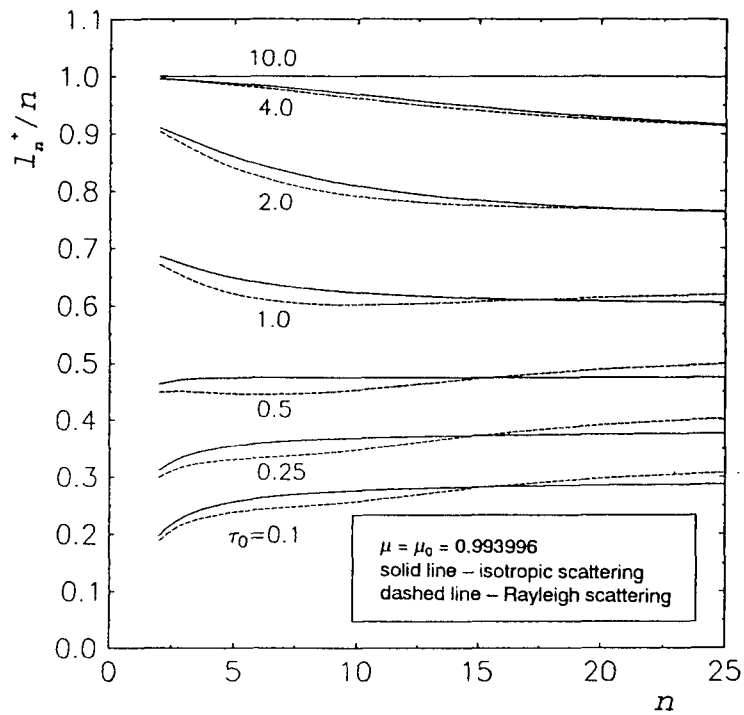
Fig. 1. Average photon path-lengths as functions of the order of scattering for almost normal reflection against optically finite atmospheres.
