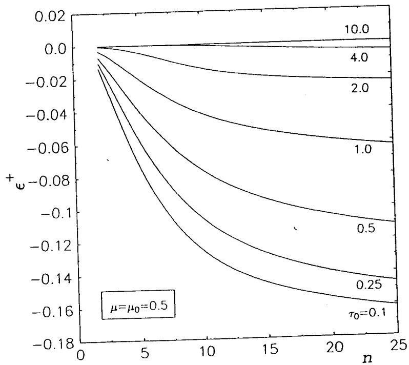
Fig. 5. Same as in Fig. 3 for different angles of incidence and reflection.
