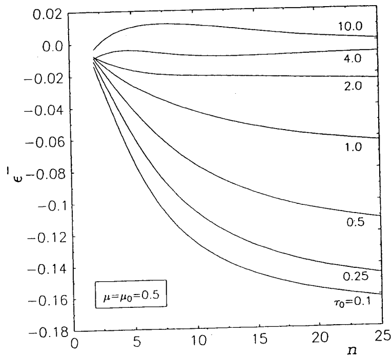
Fig. 6. Same as in Fig. 5 for transmitted radiation.
