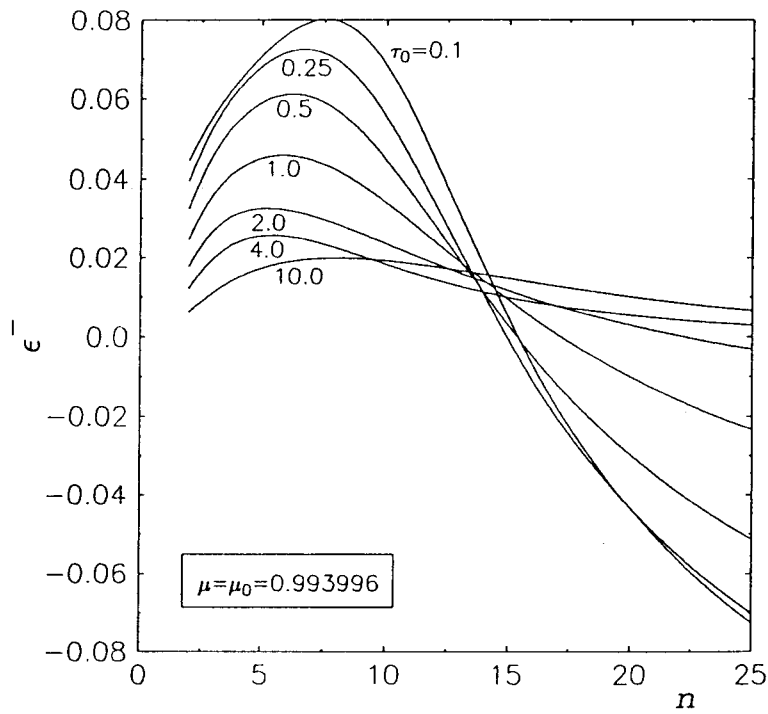
Fig. 4. Same as in Fig. 3 for transmitted radiation.
